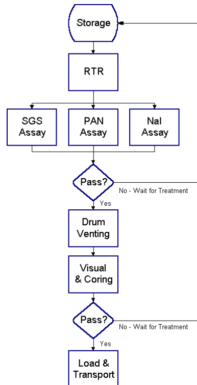
Figure 1: Flow Diagram of Waste Processing
